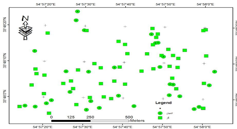
Figure 2. Distribution of the sampling points
