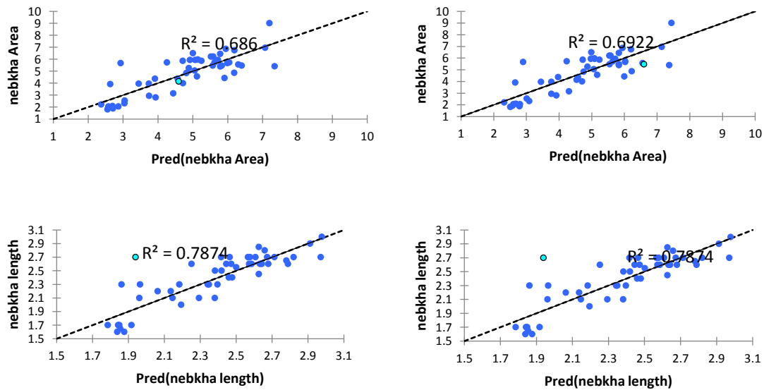
Figure 6. The relationship between the observed and predicted values via OLS and PCR in Tmarix aphylla
