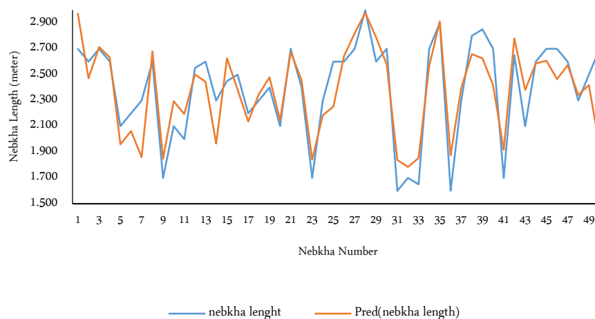
Figure 8. The relationship between the observed and predicted values of nebkha length via OLS
