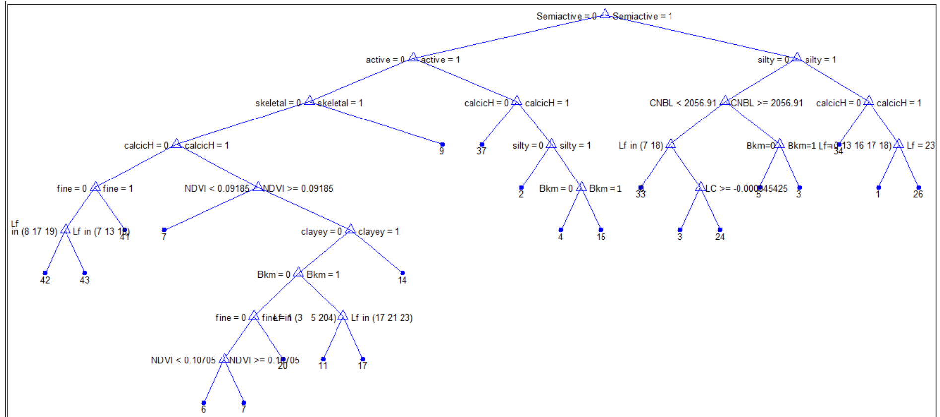
Fig. 6. Scheme of decision tree for soil family level prediction by combining auxiliary parameters and soil properties
