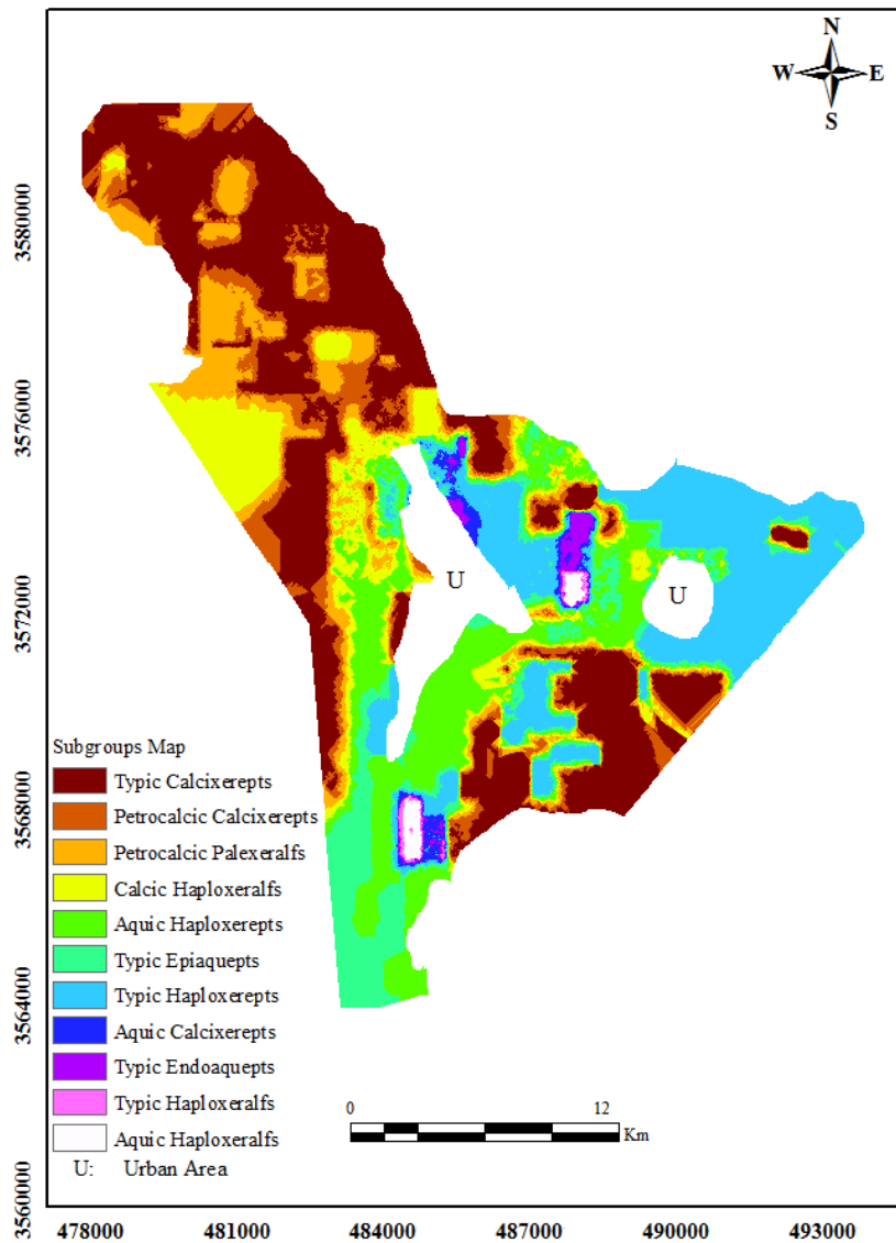
Fig. 3. Soil subgroups distribution map in the study area
