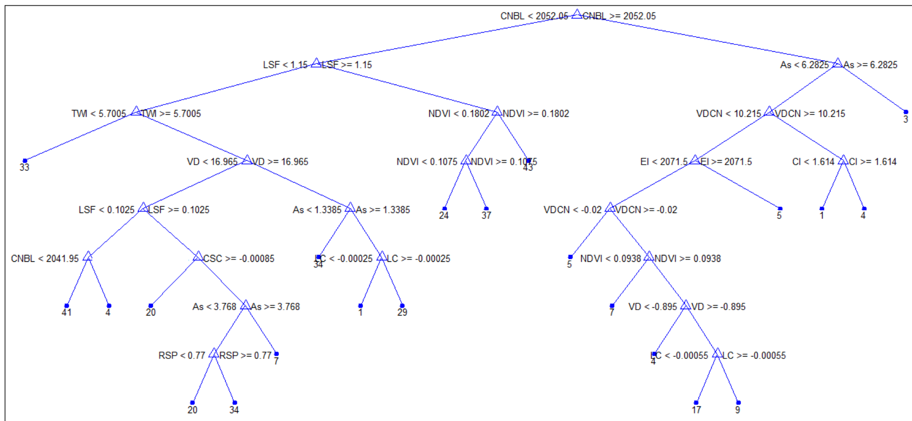
Fig. 4. Scheme of decision tree for predicting soil family classes using auxiliary parameters
