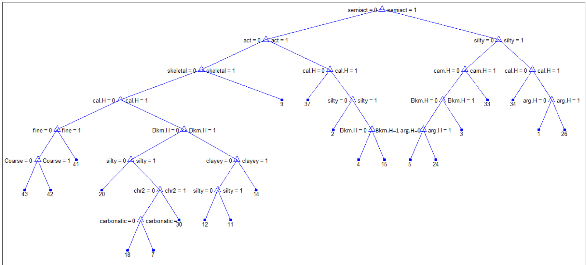
Fig. 5. Scheme of decision tree for predicting soil family classes using soil properties
