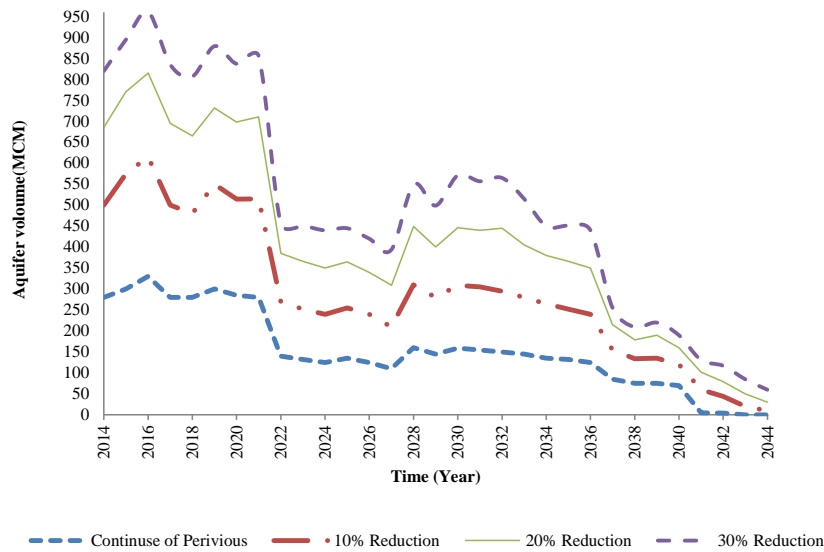
Fig. 3. WEAP outputs in different scenarios in Borojen
