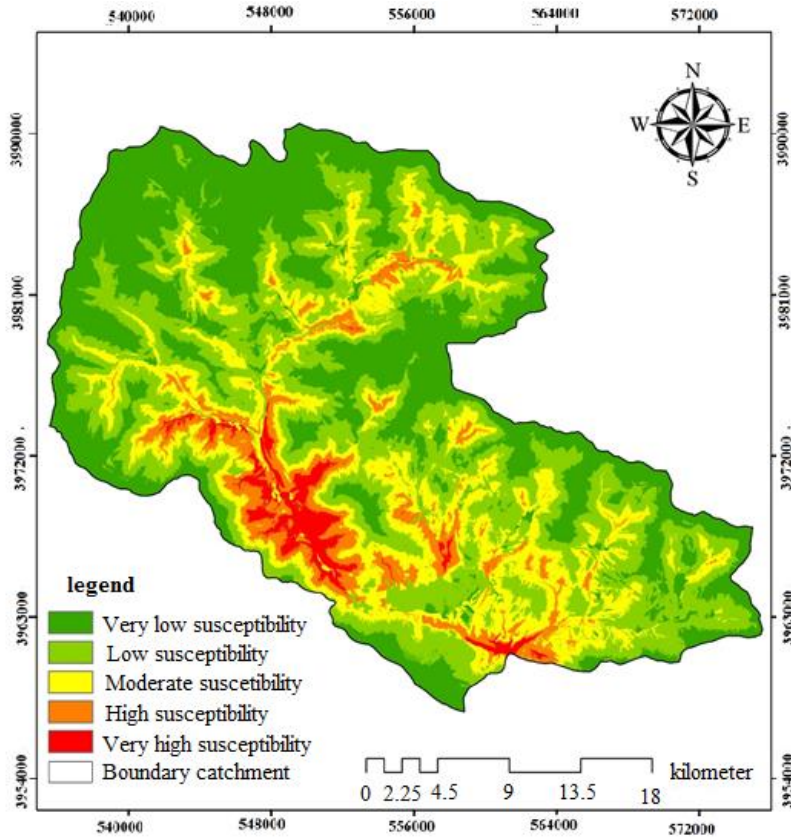
Fig. 3. Landslide susceptibility map based on LR model
