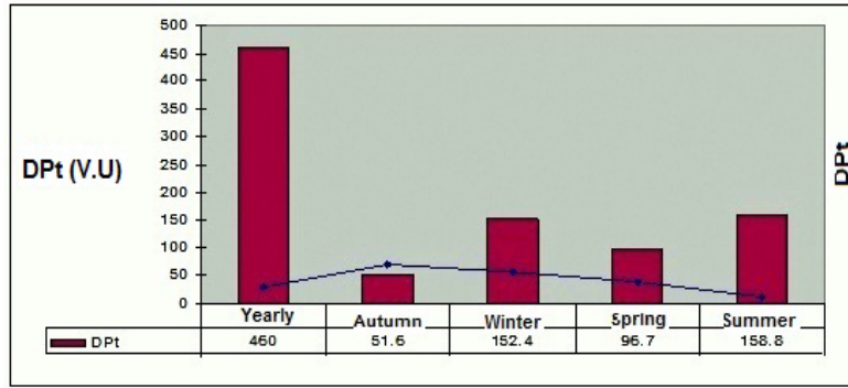
Fig. 2. Values of DP in each season
