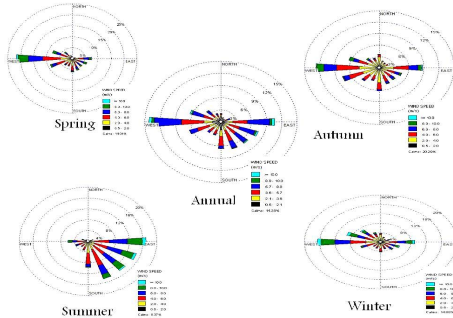
Fig. 6. Annual and seasonal wind rose (1990-2005)
