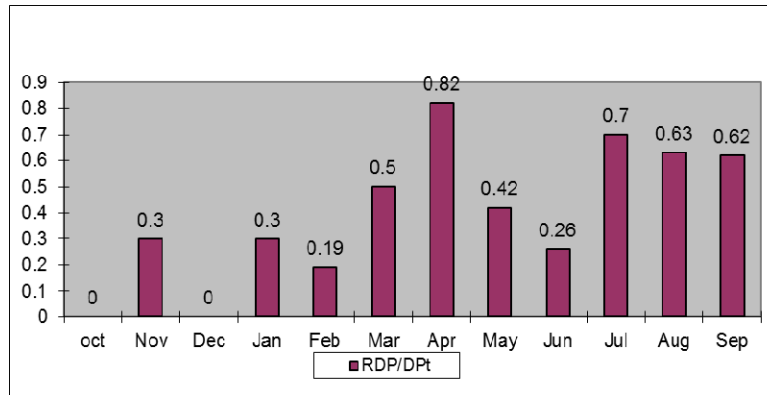
Fig. 3. Variability in wind direction in different months
