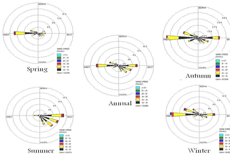
Fig. 7. Annual and seasonal storm roses (1990-2005)
