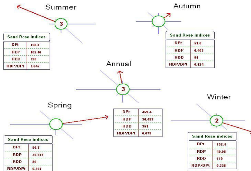
Fig. 1. Average annual, seasonal, and monthly sand DP (1990-2005)
