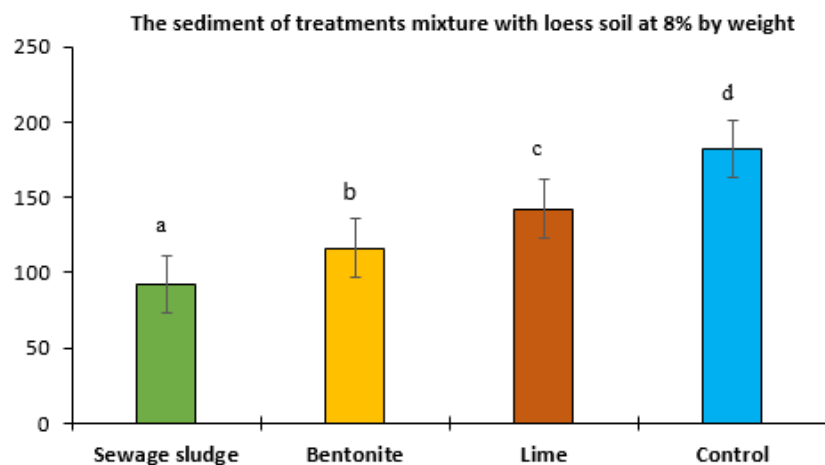
Fig. 3. Sediment produced from study treatments with a significant difference at p < 0.05 . (Different letters indicate significant differences at p < 0.05 and bars denote standard errors of the means).
