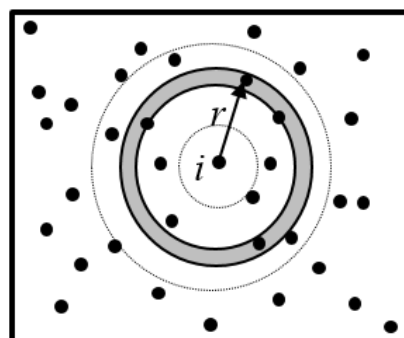
Fig. 4. Measuring plant intensity in circles with variable radius ( r ) on each plant ( i ) in O -ring function
