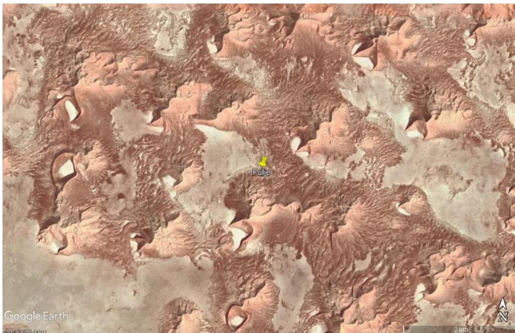
Fig. 6. Oman, South Rub' al Khali. Merged star dunes. 19°27'14.18"N, 53°38'39.30"E.. ©Google Earth, Scale bar = 2km. The difference in altitude between the peaks of the stars and the hollows is c 80 m.
