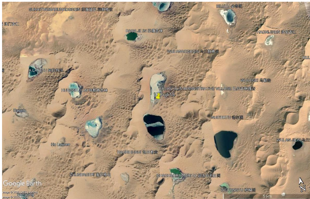
Fig. 13. China, Badain Jaran, 39°48'4.11"N, 102°25'30.58"E. ©Google Earth, Scale bar = 5 km. The relative relief is c 300 m.
