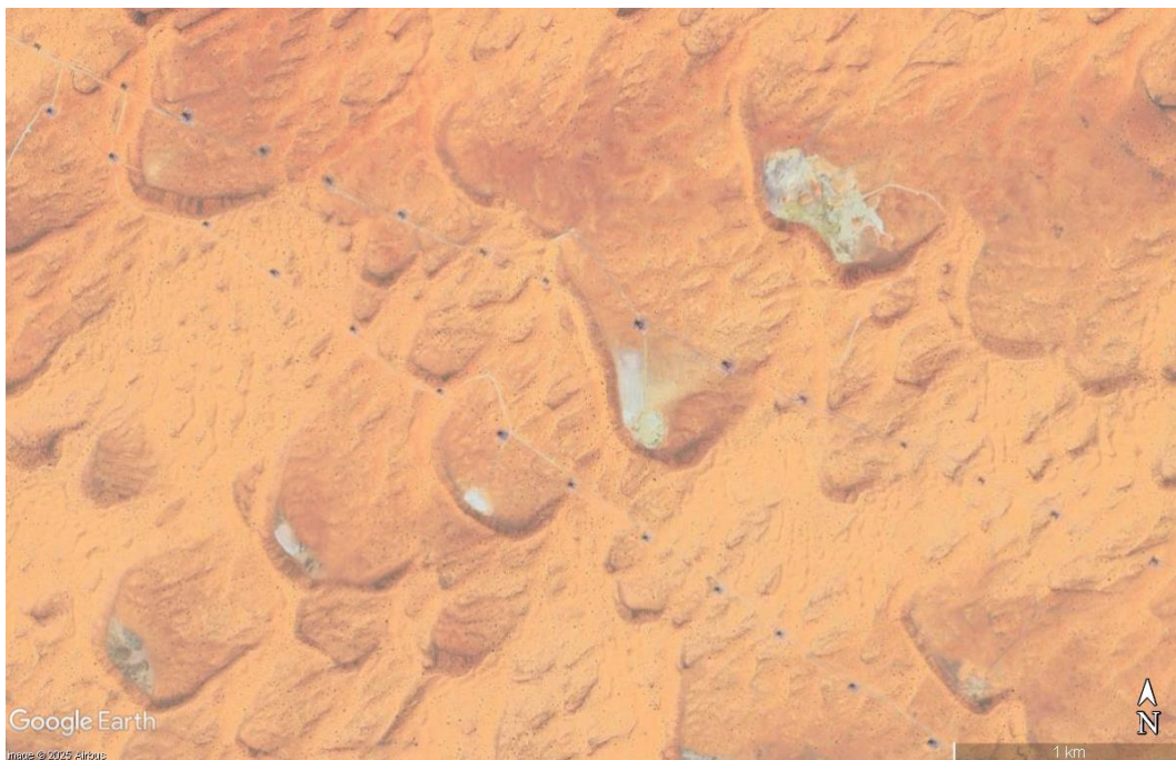
Fig 1.2. Nafud Desert, Saudi Arabia, showing fuljis in lee of barchanoid elements. 27^{\circ}54'24.68''\text{N} , 41^{\circ}21'30.75''\text{E} . ©Google Earth, Scale bar = 1km.
