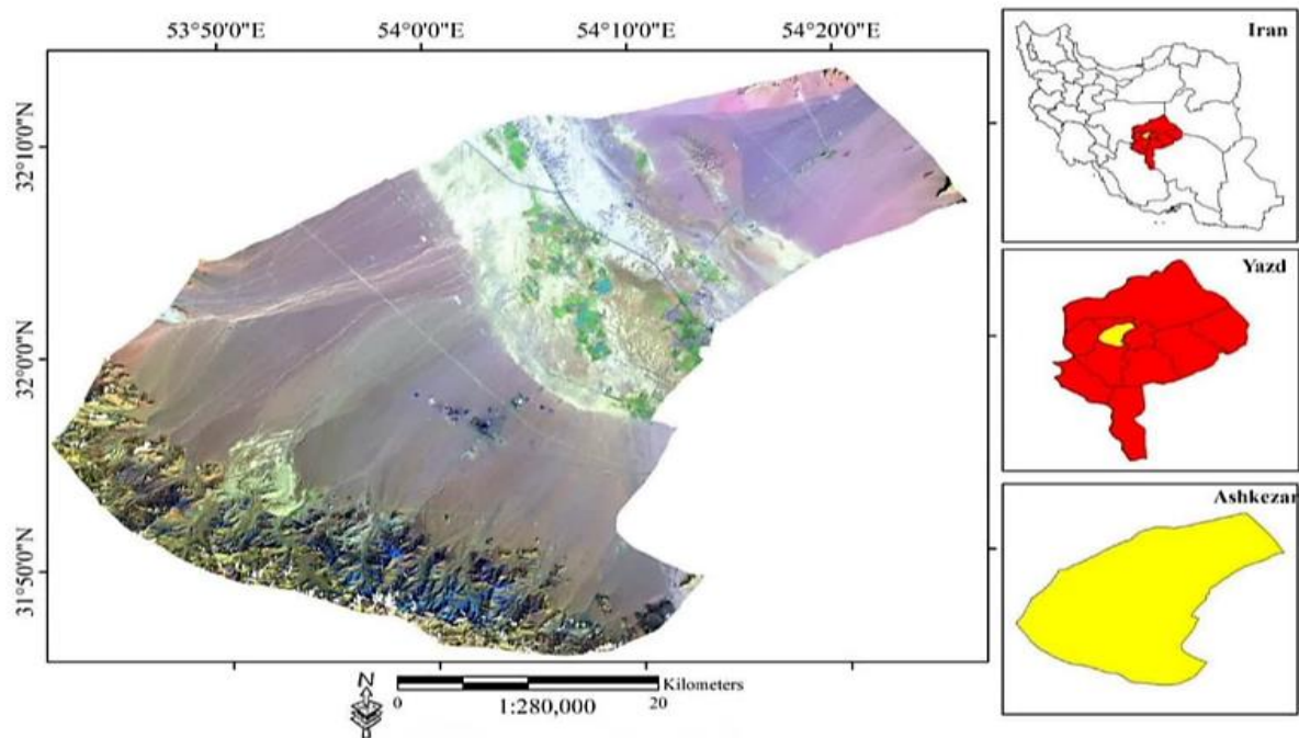
Fig 1. Location of the study area in a) Iran, b) Yazd province and, c) Landsat image
