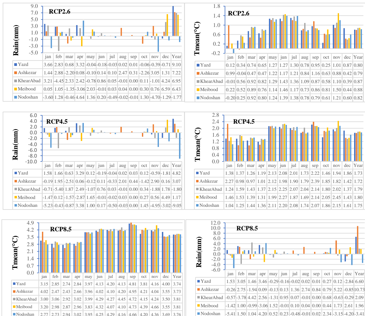
Fig. 8. Changes of predicted climate elements of all stations in the far future (2071-2100) compared to the base period in three radiative forcing scenarios (RCP8.5, 4.5, 2.6)
