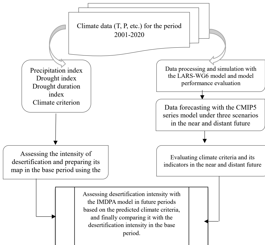
Fig. 3. Flowchart of research steps
