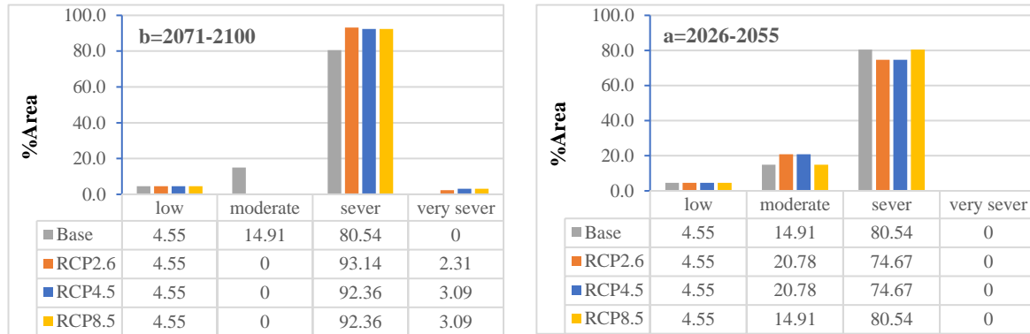
Fig. 14. Comparison of desertification risk classes of scenarios in the near future (a) and far future (b)
