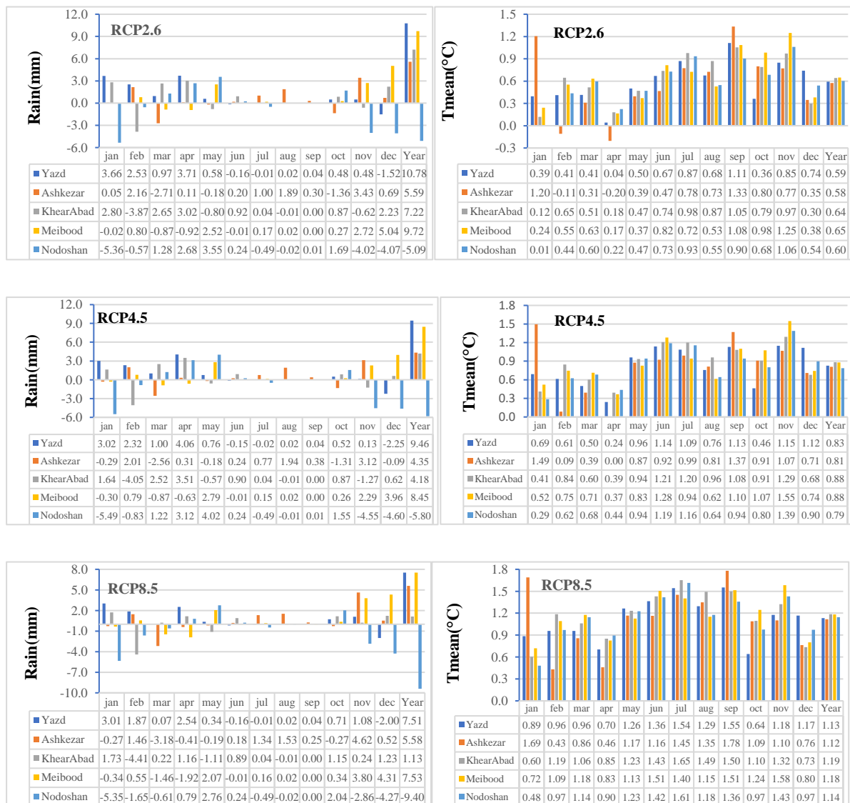
Fig. 7. The changes of the predicted climatic elements of all stations in the near future (2055-2026) compared to the base period in three radiative forcing scenarios (RCP8.5, 4.5, 2.6)
