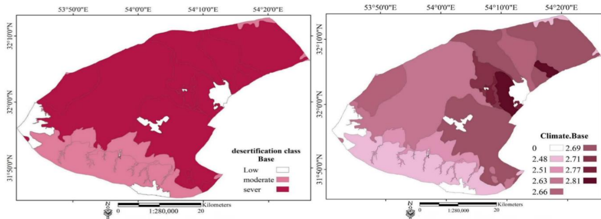
Fig. 6. Quantitative and qualitative map of the desertification risk class in the base period
