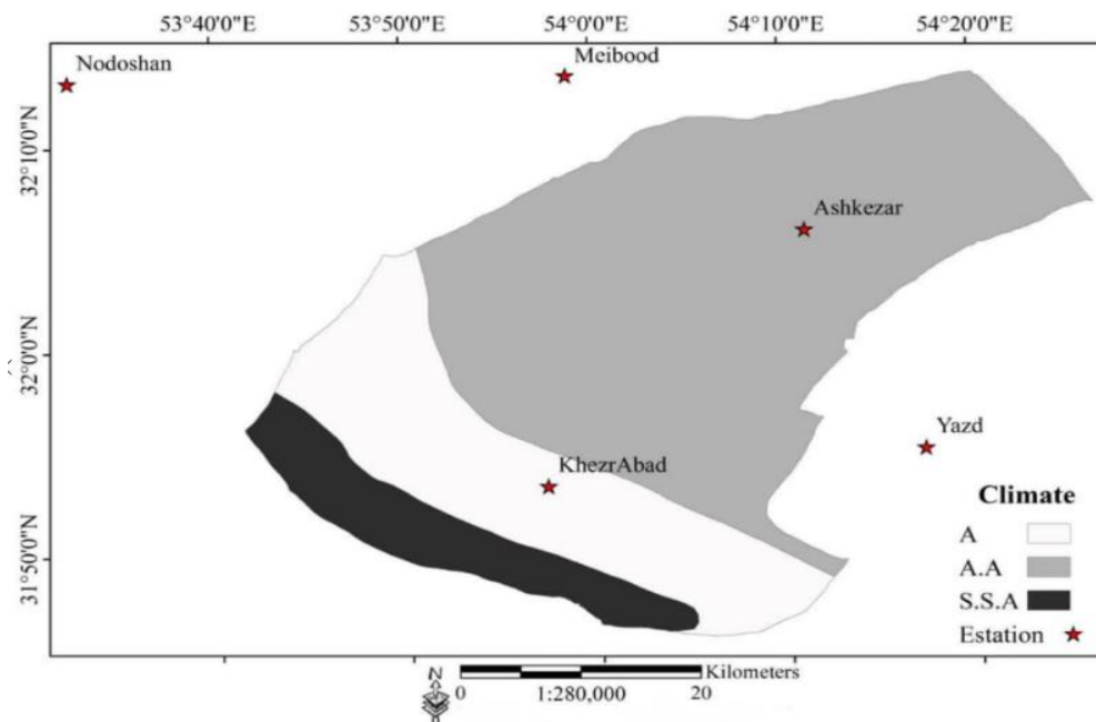
Fig 2. Climate classification map of the study area based on Selianinov method
