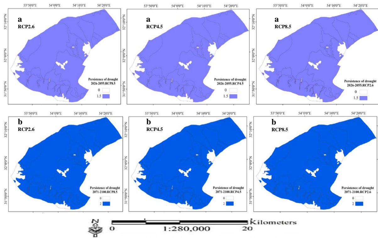
Fig. 11. Intensity of desertification, index of drought continuity for the period 2055-2026 (near future, a), and 2100-2071 period (far future, b) in RCP2.6, 4.5, 8.5 scenarios
