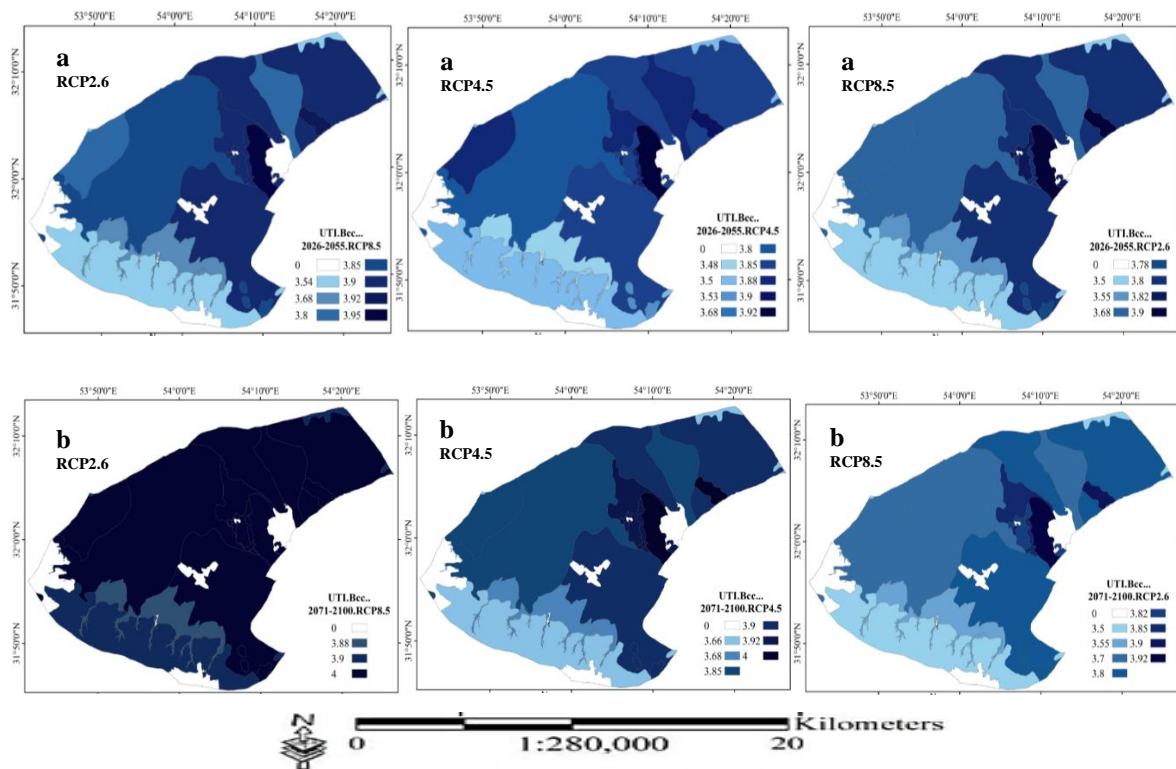
Fig. 10. Intensity of desertification of drought index for the period 2055-2026 (near future, a) and 2100-2071 period (far future, b) in RCP2.6, 4.5, 8.5 scenarios
