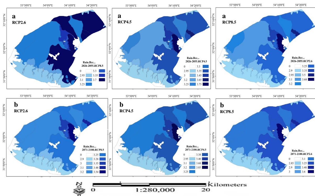
Fig. 9. Desertification intensity of rainfall index for the period 2055-2026 (near future, a) and 2100-2071 period (far future, b) in RCP2.6, 4.5, 8.5 scenarios
