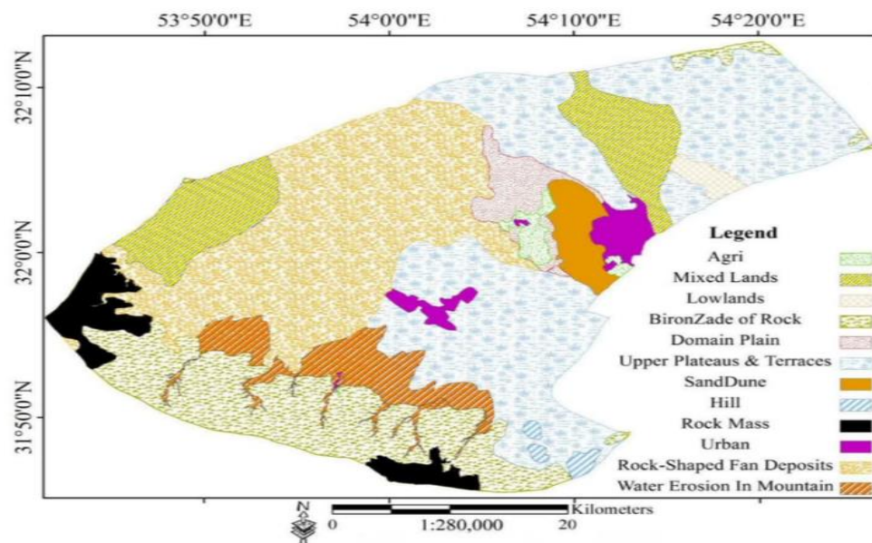
Fig. 4. Works-unit map in Northwest of Yazd (geomorphological Facies)
